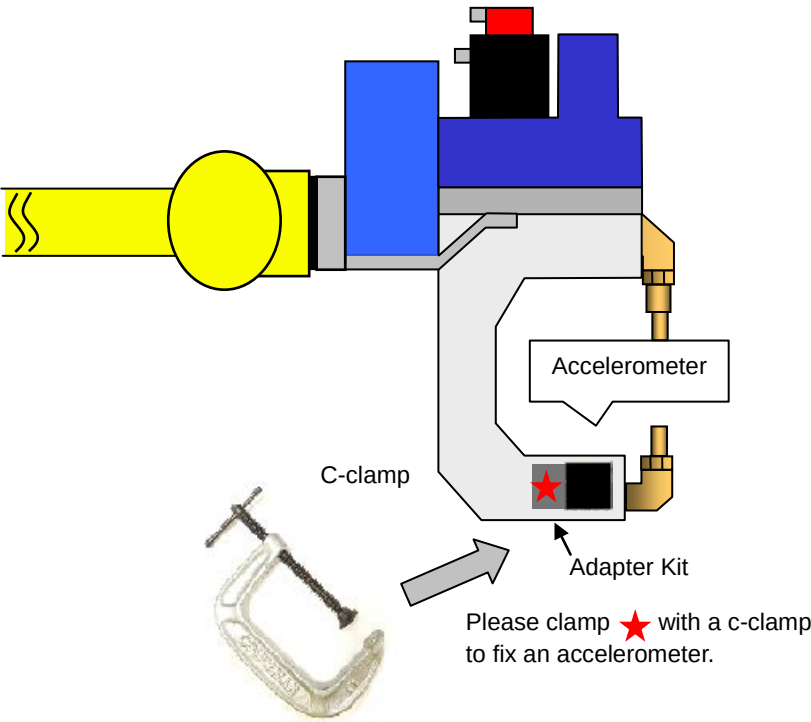
Fig. 2.1.2 (h) Clamping an Accelerometer with a C-clamp Kit
