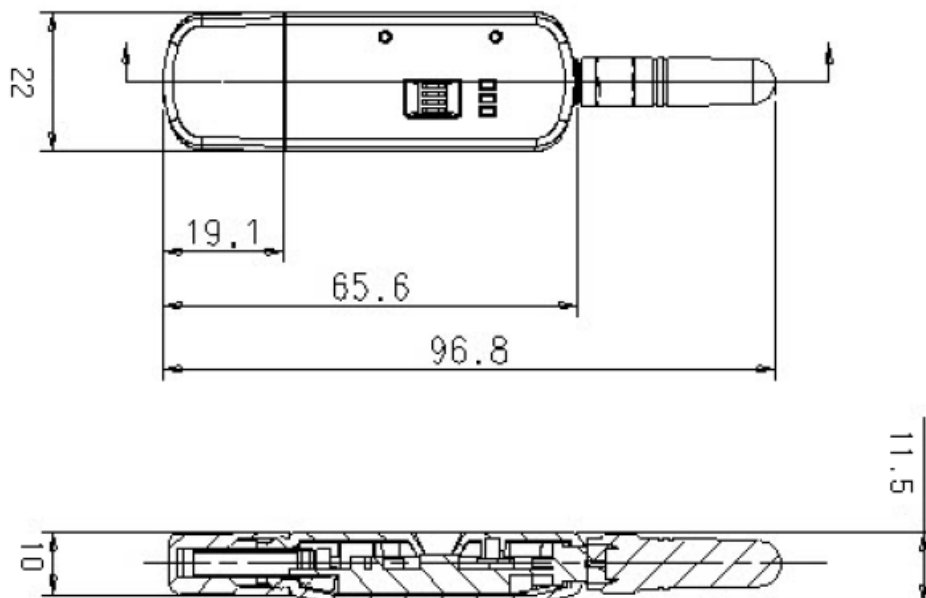
Fig. 2.1.2 (b) Dimensions of the USB receiver
